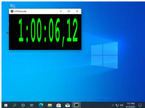
Window
